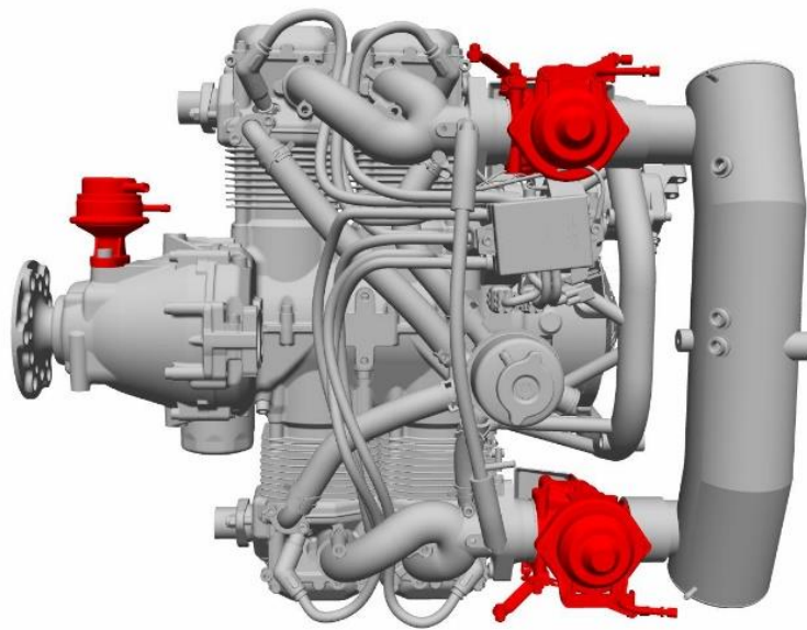
Fuel System
